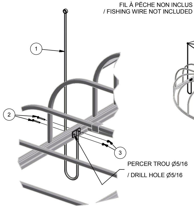
DETAIL A
